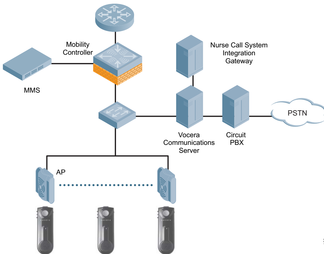
Figure 13 Vocera Integration Into Alcatel-Lucent Network
