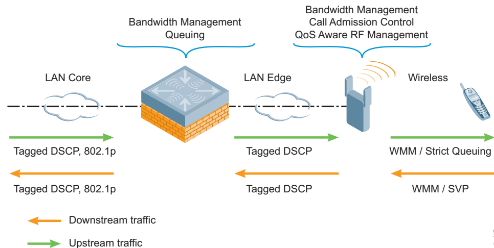
Figure 2 End-to-End QoS
