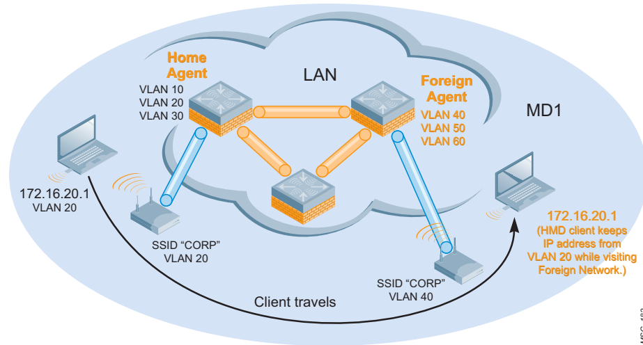
Figure 9 L3 Mobility
